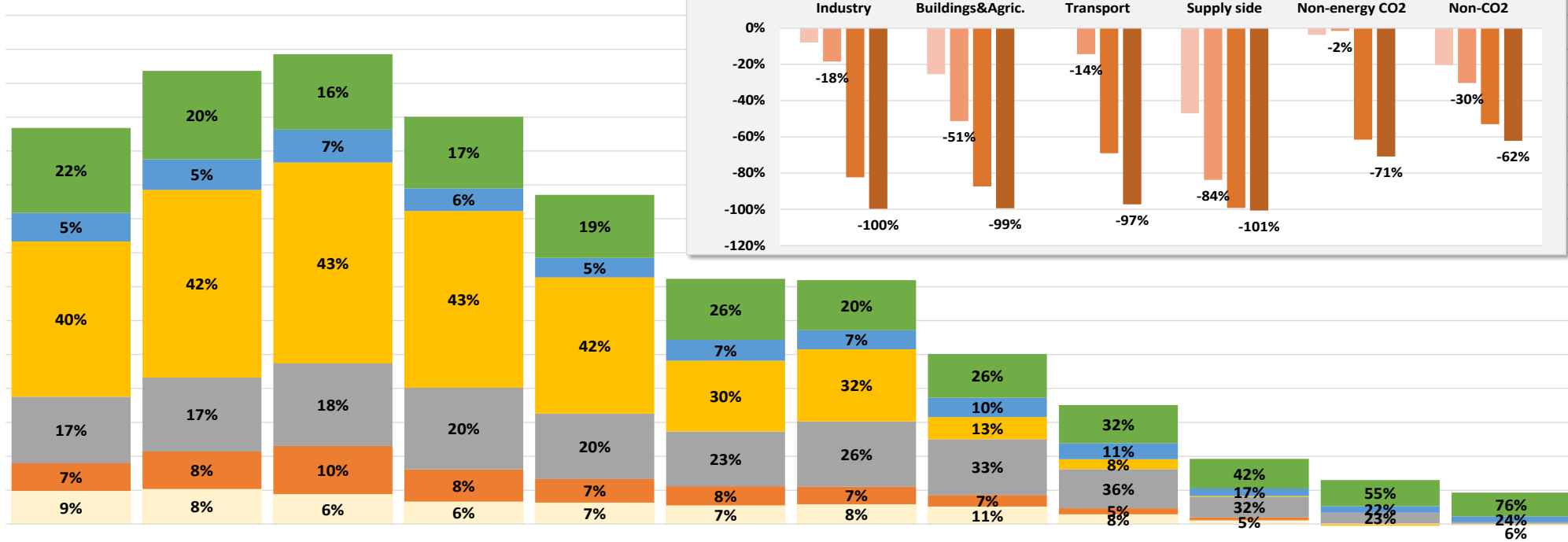
NECP AB - Greenhouse Gas Emissions (excl. LULUCF)
